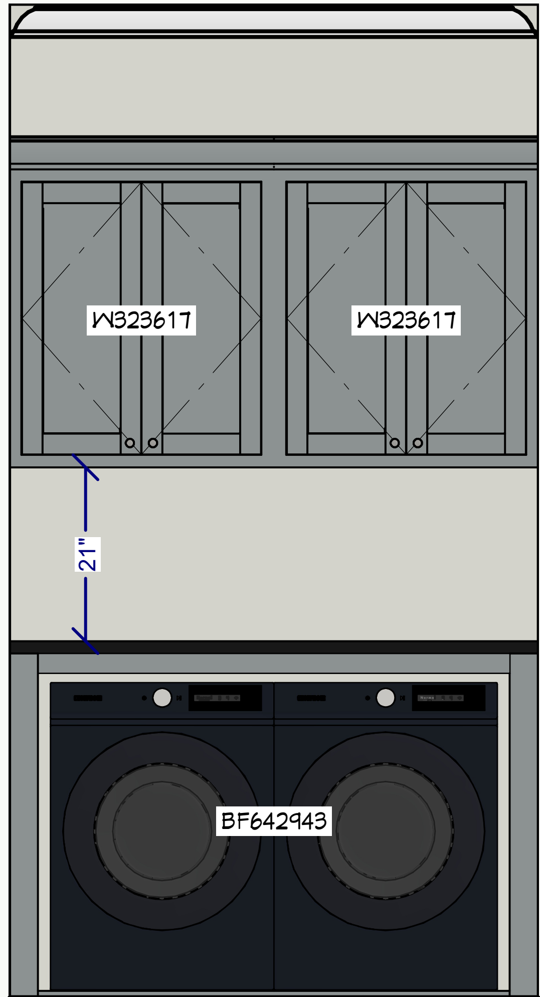
ELEVATION: LAUNDRY ROOM 1
